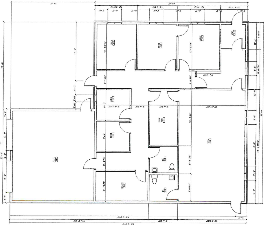
1 LEVEL 1 1/8" = 1'-0"
